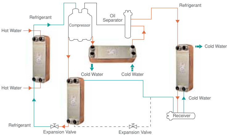
Hot Loop Dried Circuit
