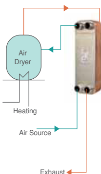
Hot Loop Dried Circuit
