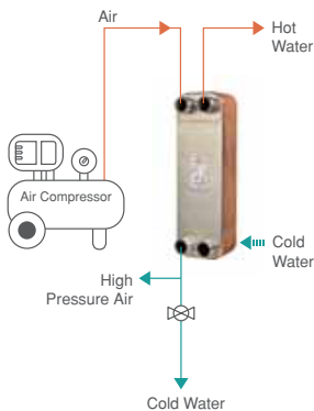
Air-Drying Cooler
