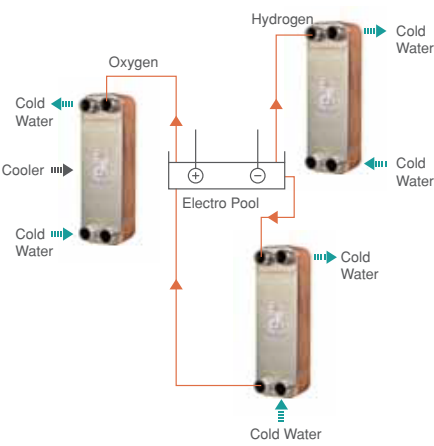
Electrolysis Process Circuit
