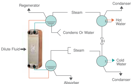
Absorbed Refrigeration
